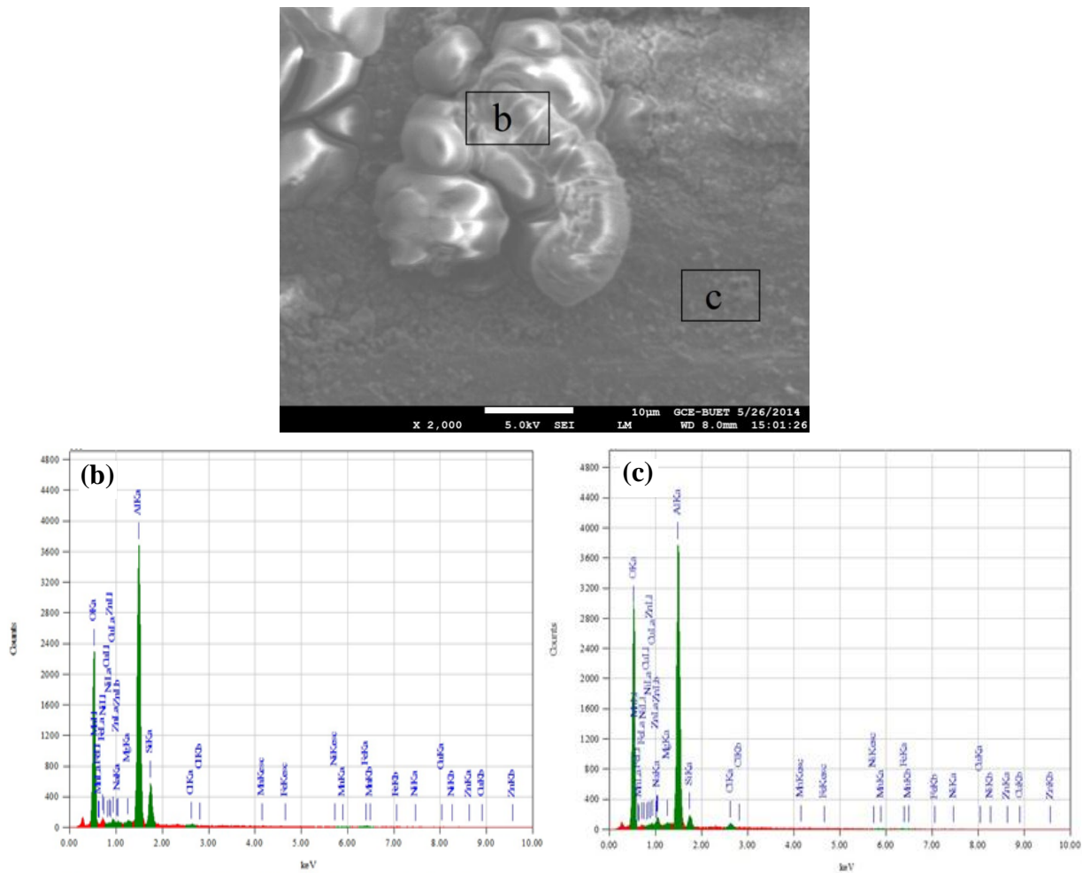
Figure 9. SEM Images and EDX of Piston after Wear in Corrosive Environment at 1.4 MPa Applied Pressure and Sliding Distance of 4200 m.
